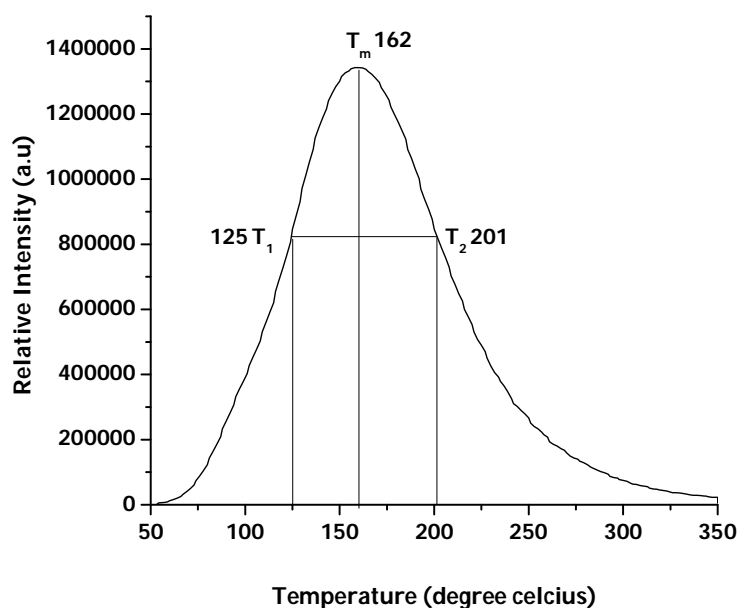
Figure: 2. The TL glow curve of \text{Sr}_2\text{B}_2\text{O}_5:\text{Tb}^{3+} phosphor irradiated by \gamma -rays at room temperature.
