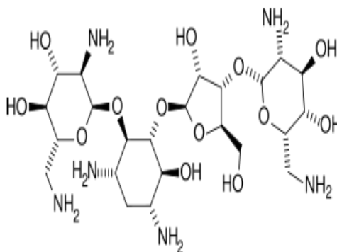
Fig. 1 Chemical structure of Neomycin
