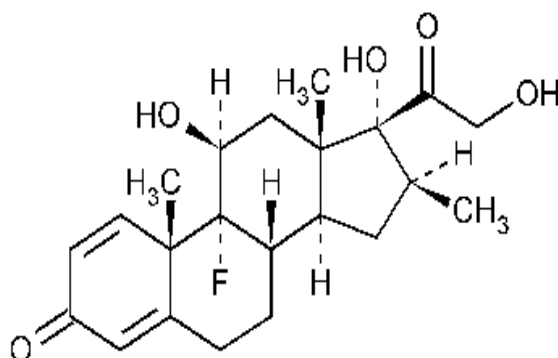
Fig. 1 Chemical structure of Betamethasone
