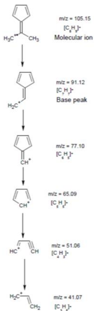
Scheme.1 Fragmentation pattern of 5-(1-methylethylidene)-1, 3-cyclopentadiene
