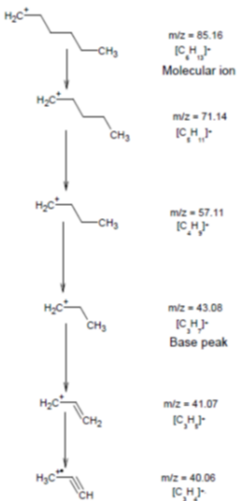
Scheme.7: Fragmentation pattern for Hexane
