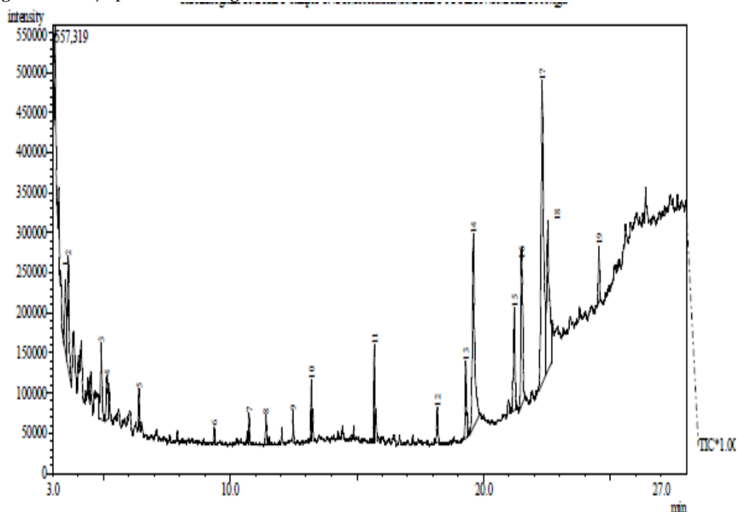
Figure 2: Chromatogram of Ethanol Extract of Whitfieldia lateritia Leaf.
