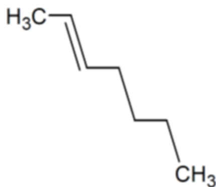
Figure.15 Hept-2-ene
