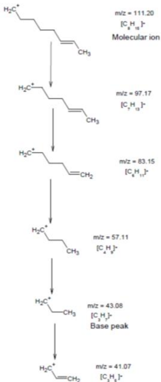
Scheme.13 Fragmentation for Oct-2-ene
