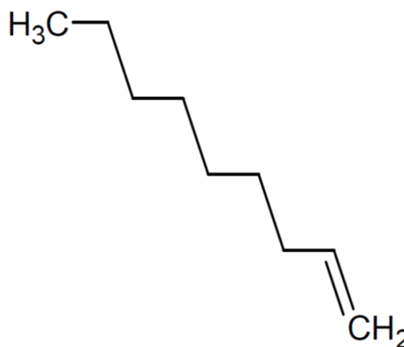
Non-1-ene
