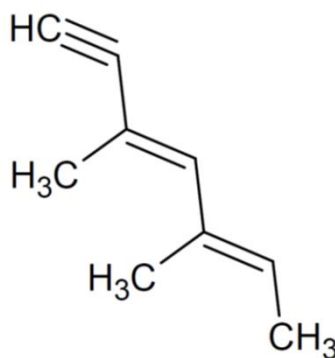
Figure.5: 3,5-dimethylhepta-3,5-dien-1-yne
