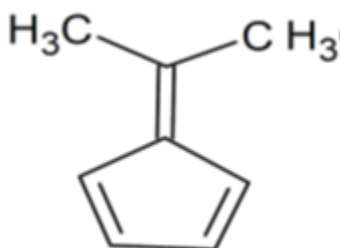
5-(1-methylethylidene)-1,3-cyclopentadiene
