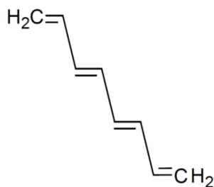
Figure.3:Octa-1,3,5,7-tetraene
