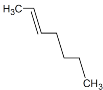
Hept-2-ene
